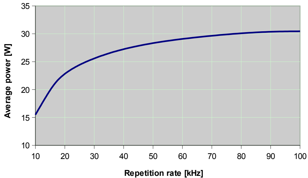
Sol 30W 1064nm: Average Power
