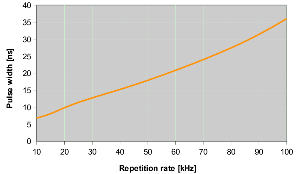
Sol 30W 1064nm: Pulse Width
