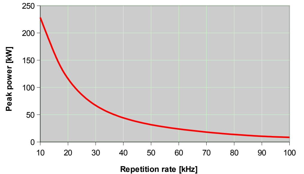
Sol 30W 1064nm: Peak Power
