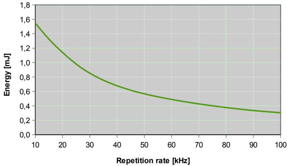
Sol 30W 1064nm: Pulse Energy
