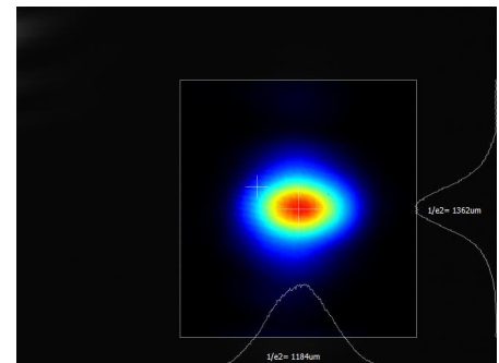
Typical near field (0.45 m from output aperture) beam profile. Non-circularized beam of a 0975 nm direct diode laser.
