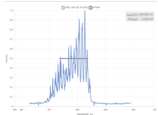
Typical spectrum of 0450 nm diode laser. Measured with 10 pm resolution.
