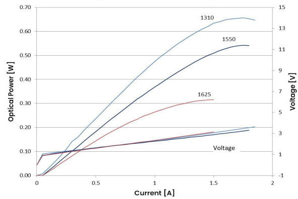
TO9: Single Mode 2.5 mm CL, Uncapped
