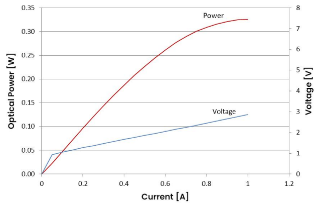
TO9: Single Mode 1650nm, 1.25 mm CL ,Capped
